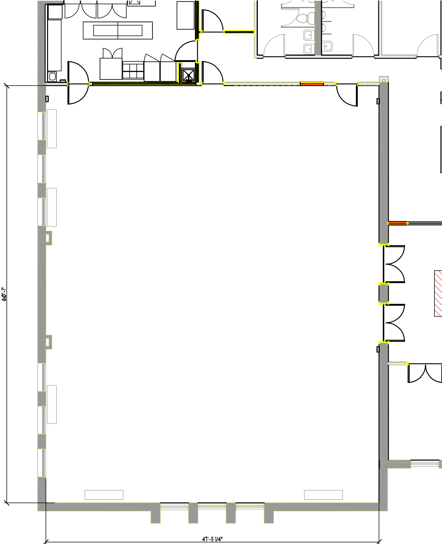
MULTIPURPOSE ROOM FLOOR PLAN 1/8" = 1'-0"
